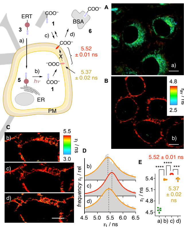
Figure 3. FLIM images of HK cells after (A) addition of ER PhotoFlipper 3 (a, 2.5 \mu M, 15 min), (B, Cb) irradiation (b, \lambda = 365 nm, 2.5 min), (Cc) subsequent addition of 1 (c, 1 \mu M, 2 min), and (Cd) treatment with media containing BSA (d, serum 10%). Scale bar: 10 \mu m. (D) FLIM histogram associated with the \tau_1 component of 1 in stages b-d in C. (E) Fluorescence lifetimes of flipper probes in the four different stages a-d in A-C; statistical significance was determined using Student's t-test, ns: p > 0.05 , *: p < 0.05 , **: p < 0.005 , ***: p < 0.0005 , ****: p < 0.0001 (unpaired from a to b, paired from b to c and c to d).
