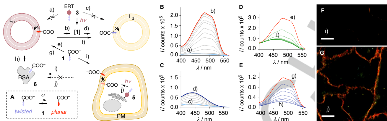
Figure 2. (A) Mode of action of 1 , \sigma = compressive force. (B) Excitation spectra of 3 (100 nM, \lambda_{em} = 600 nm) in SM/CL LUVs (75 \mu M) at 25 °C before (light blue) and after up to 20 min of bulk irradiation at \lambda = 365 nm (grey to red). (C) Same as (B) in DOPC LUVs (75 \mu M) with final spectrum in dark blue (c-d). (D) Excitation spectra of 1 (100 nM, \lambda_{em} = 600 nm) in SM/CL LUVs (75 \mu M) 0 min (e, red), 0.5 to 5 min (f, green) after addition of DOPC LUVs (75 \mu M). (E) Excitation spectra of 1 (40 nM, \lambda_{em} = 600 nm) in SM/CL LUVs after addition of 0 (g, red), 0.25 to 20 \mu M (h, blue) BSA. (F) FLIM image of 1 (1 \mu M, 15 min) in HK cells after washing with BSA (serum 10%, 3 x 1 mL, i) and (G) of 3 (5 \mu M, 15 min) after irradiation ( \lambda = 365 nm, 3 min) and washing with BSA (serum 10%, 3 x 1 mL, j). Scale bar: 10 \mu m.
