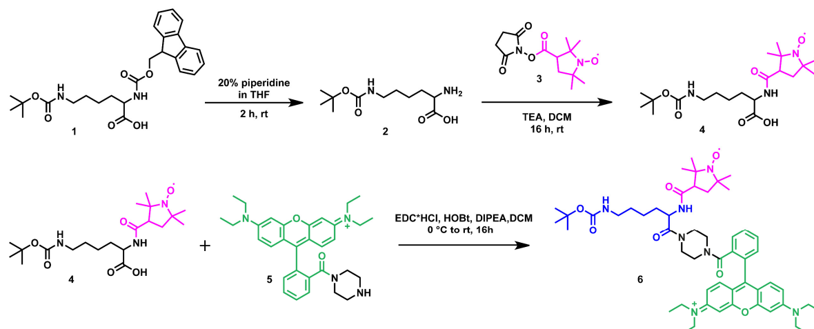
Figure 2. Scheme of DL synthesis. PCA ( 3 ) and Rhodamine B-piperazine ( 5 ) were covalently linked to Fmoc-Lys(Boc)-OH ( 1 ) yielding the DL conjugate ( 6 ). ( 2 ) deprotected Lys(Boc)-OH, ( 4 ) Boc-Lys-PCA.
