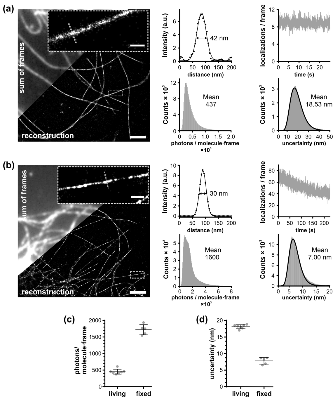
Figure 3. SMLM imaging of microtubules in living and fixed U-2 OS cells stained with HMSiR-tubulin (3): (a) Living cells. (b) Fixed cells. Zoom-in on a single microtubule and intensity profile along the dashed line are shown, together with the corresponding fitting to the Gaussian function. Scale bar 2 \mu\text{m} ; zoom-in 0.5 \mu\text{m} . The movies used for reconstruction are in Supplementary Videos 1 and 2. Fluorophore properties (histograms of localization uncertainty and photon count per molecule per frame and bleaching time-course) are shown. Fitting to log-normal distribution is shown as a thick line. Comparison of photon count per molecule per frame (c) and localization uncertainty (d) in living and in fixed samples. The data is from 6 and 7 fields of view, from 2 independently prepared samples.
